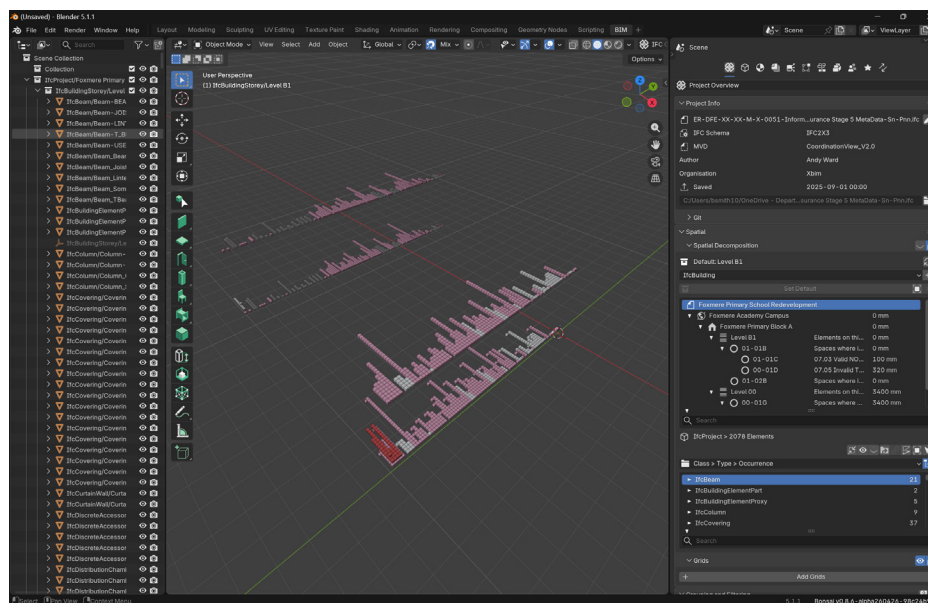
Figure 6: IFC-SPF loaded
