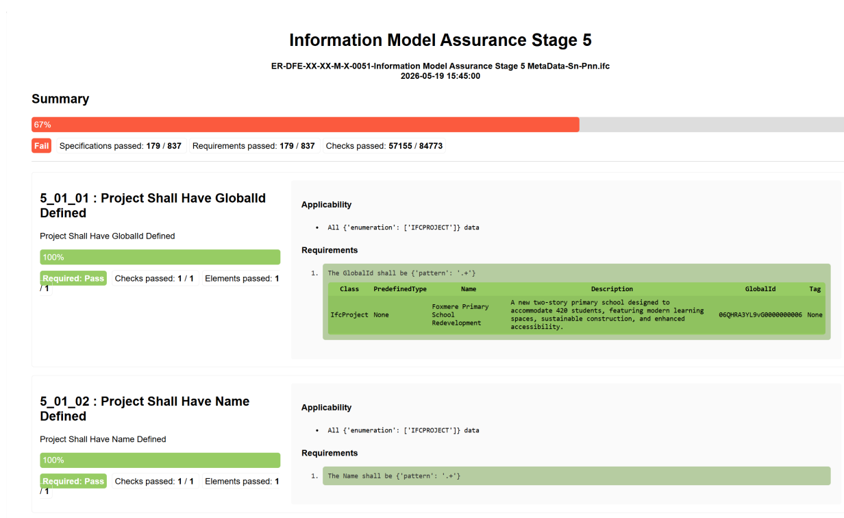
Figure 9: Result output
